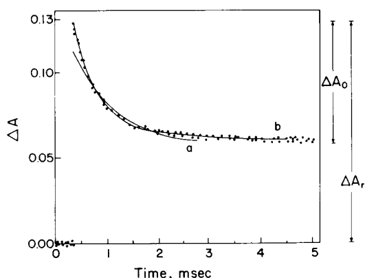
FIG. 1. The change of absorbance with time for oxygen binding to the valence hybrid in the presence of IHP. Curve a is a computer best fit using a simple first order kinetic expression (Equation 3). Curve b is a best fit of the same data points using a biphasic kinetic expression (Equation 4). \lambda = 435 \text{ nm} ; [\text{MetHb}] = 20 \mu\text{M} tetramer; [e_{aq}^-] = 5 \mu\text{M} ; [O_2] = 83 \mu\text{M} ; [\text{phosphate}] = 0.02 \text{ M} , pH 7.5.
