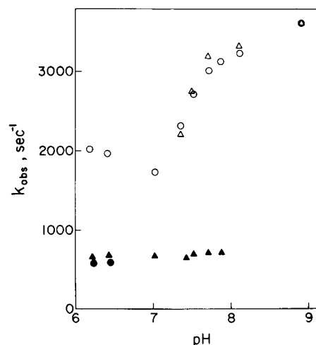
FIG. 2. pH dependence of the pseudo-first order rate constants for the binding of oxygen to the valence hybrid. In the absence of IHP: k , \circ , \bullet ; in the presence of IHP: k^f , \triangle ; k^s , \blacktriangle .
