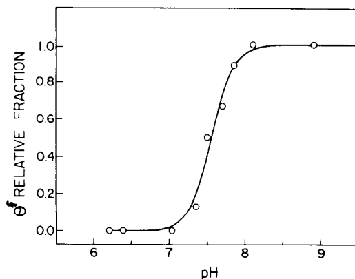
FIG. 4. pH dependence of the relative contribution ( \theta^f ) of the fast-reacting valence hybrid to the overall reaction. ( \theta^f = \Delta A_o^f / \Delta A_o ). The values of \theta^f have been calculated from the experimental data shown in Table I. The solid line is a best fit of the Hill equation \theta^f = 1 / (1 + 10^{n(pK - pH)}) to the experimental values of \theta^f .
