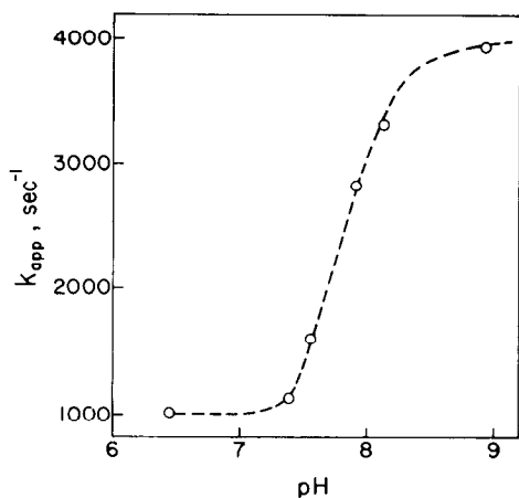
FIG. 3. pH dependence of k_{app} for the reaction of oxygen with the valence hybrid in the presence of IHP. All experimental conditions are as in Fig. 2. The apparent rate constants k_{app} have been evaluated from the reaction curves using single first order rate equations.
